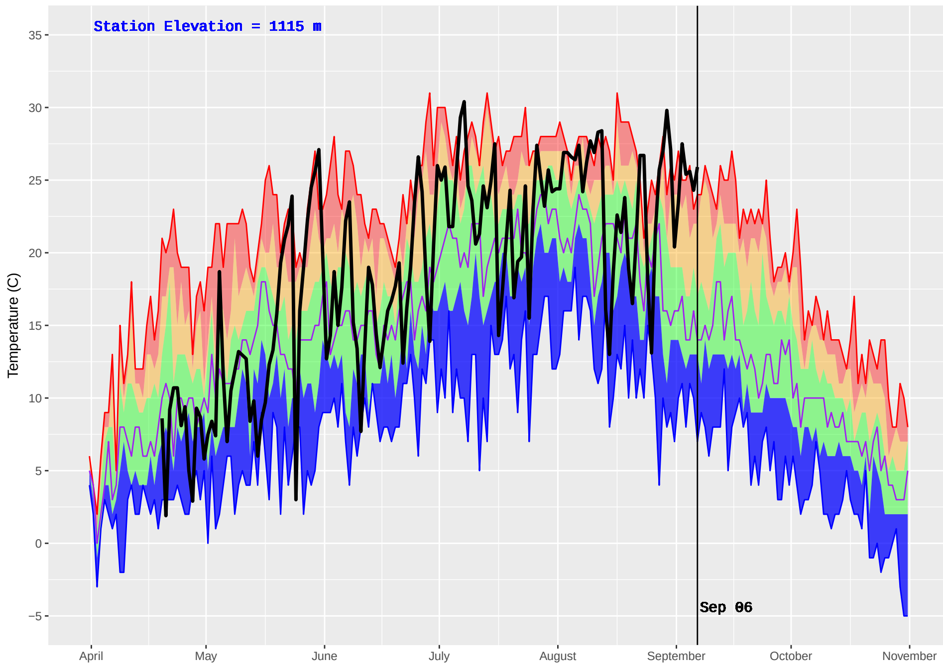
SICAMOUS (882) : Historical (2004–2016) and Current (2017) Noon Temperature
