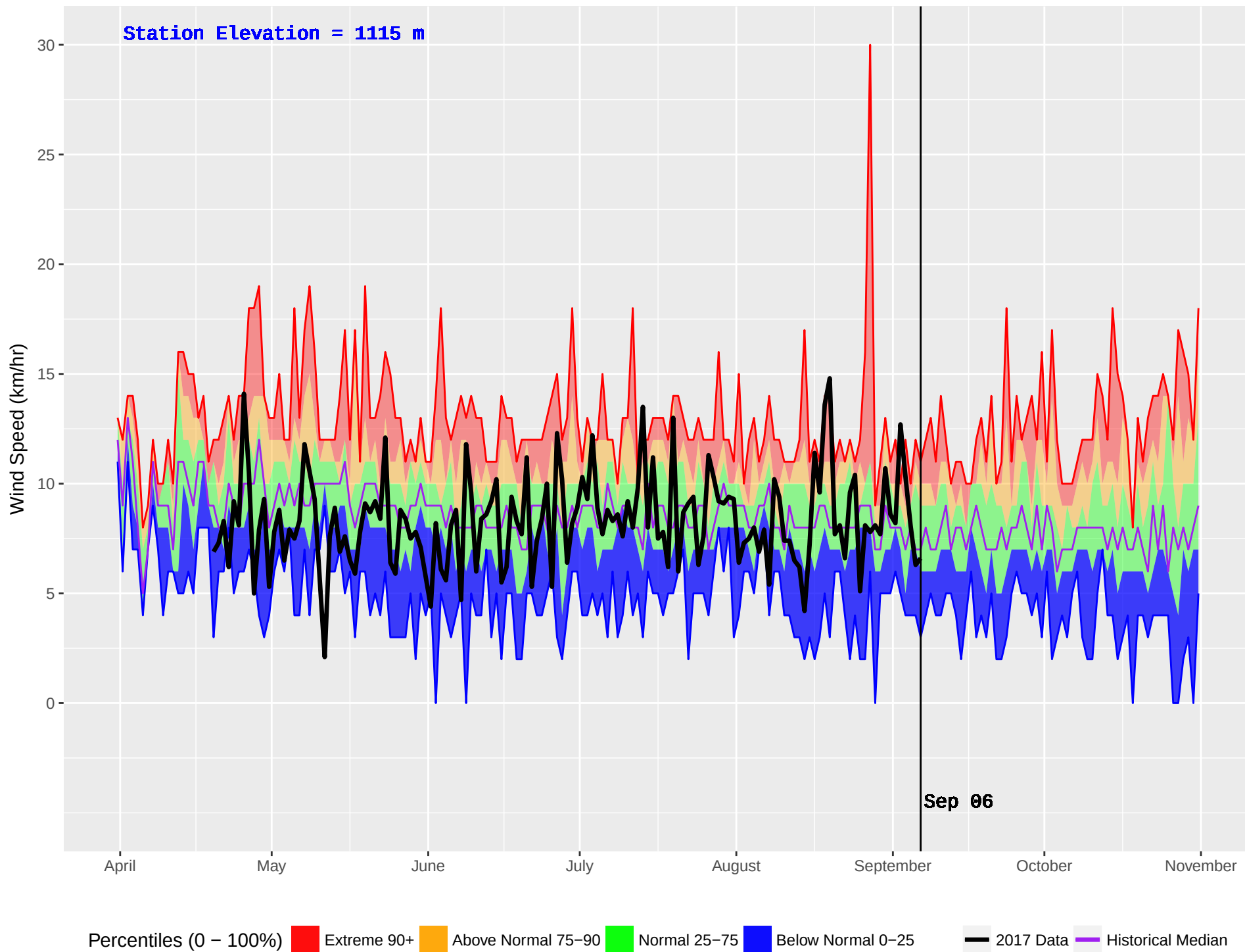
SICAMOUS (882) : Historical (2004–2016) and Current (2017) Noon Wind Speed
