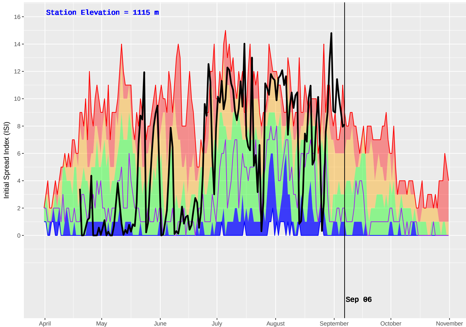
SICAMOUS (882) : Historical (2004–2016) and Current (2017) Noon Initial Spread Index (ISI)
