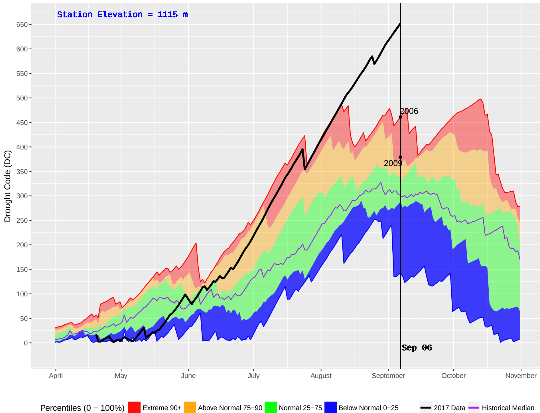
SICAMOUS (882) : Historical (2004–2016) and Current (2017) Noon Drought Code (DC)
